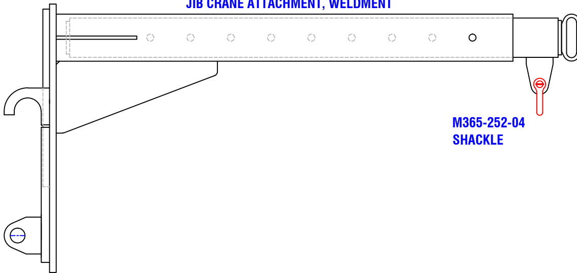
M365-252-02 JIB CRANE ATTACHMENT, WELDMENT
